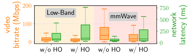
Figure 6: Impact of HO and radio band on the QoE of volumetric video streaming.
