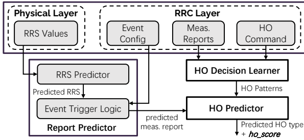
Figure 17: Design of HO prediction system Prognos.
