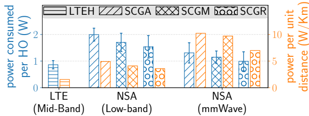
Figure 10: Comparing power consumption of HOs in Low-Band NSA 5G vs. mmWave NSA 5G vs. Mid-Band LTE.
