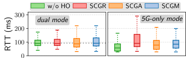
Figure 7: TCP (BBR) RTT during HO in two NSA deployment modes.
